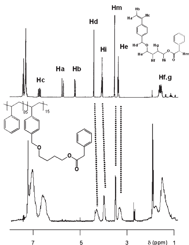
Figure 2. Comparison between the ^1\text{H} NMR (200 MHz, \text{CDCl}_3 ) spectra of monomer 2c and polymer 5C .
