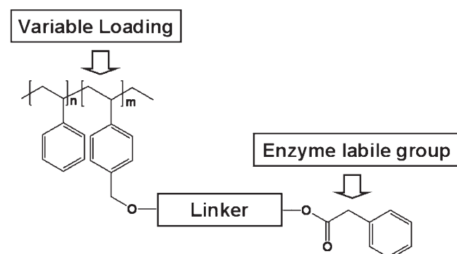
Figure 1. Design scheme for the linear polymers described in this paper.
