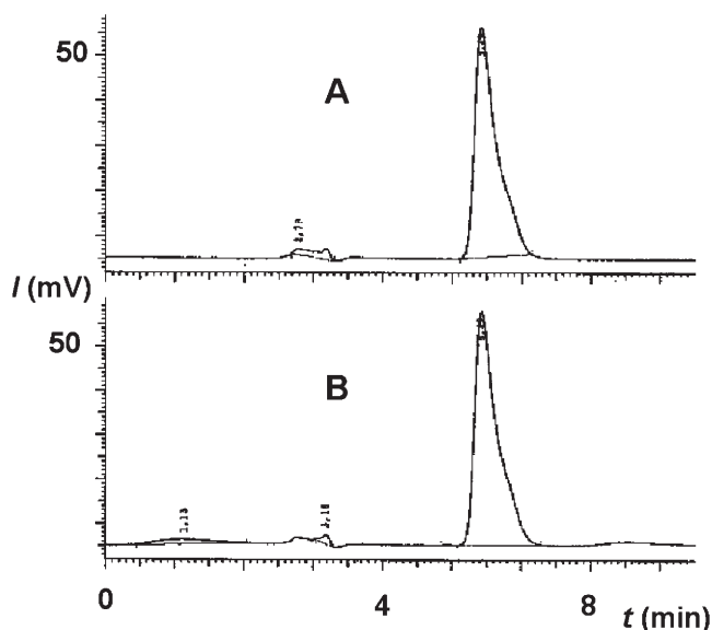
Figure 3. Reverse phase HPLC chromatograms of: A ) phenylacetic acid in the hydrolysis reaction mixture at the end of the reaction; B ) a 0.6 mM standard solution of phenylacetic acid used for the calibration curve.
